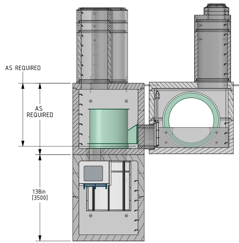
SECTION B-B
